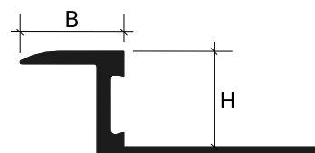
Brass B = 3/8" - 10 mm
