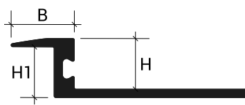
Aluminum B = 19/64" - 7.5 mm H = H1
